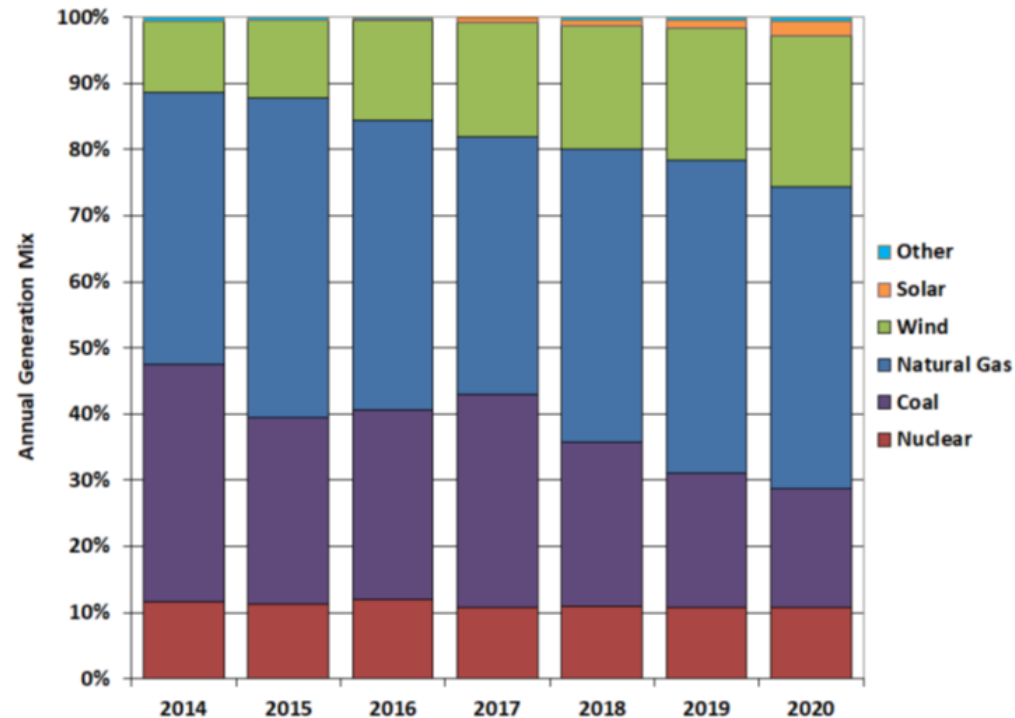
Figure 16: Annual Generation Mix in ERCOT
