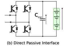
(b) Direct Passive Interface
