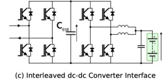
(c) Interleaved dc-dc Converter Interface
