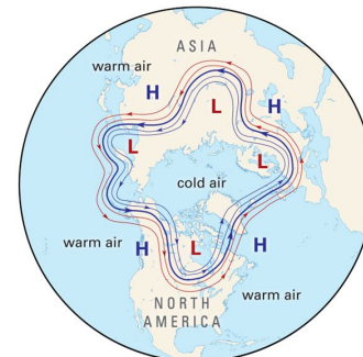
2. Waves forming in polar vortex
