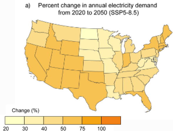
Figure 5.2. Due to climate change, electricity demand is projected to increase over this century.
