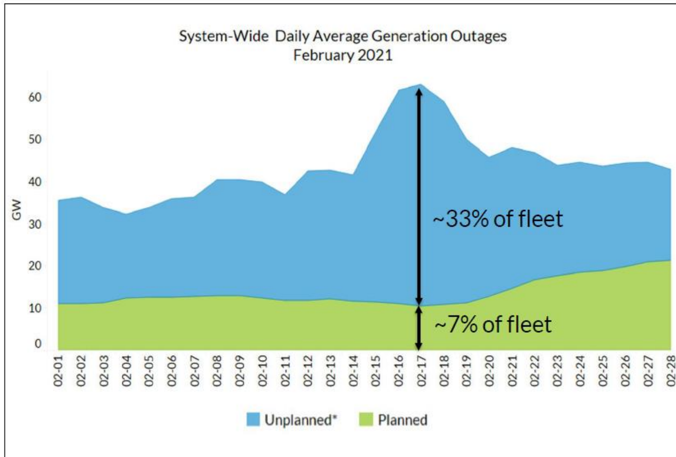
Daily Average (GW) Unplanned Generation Outages February 17, 2021
