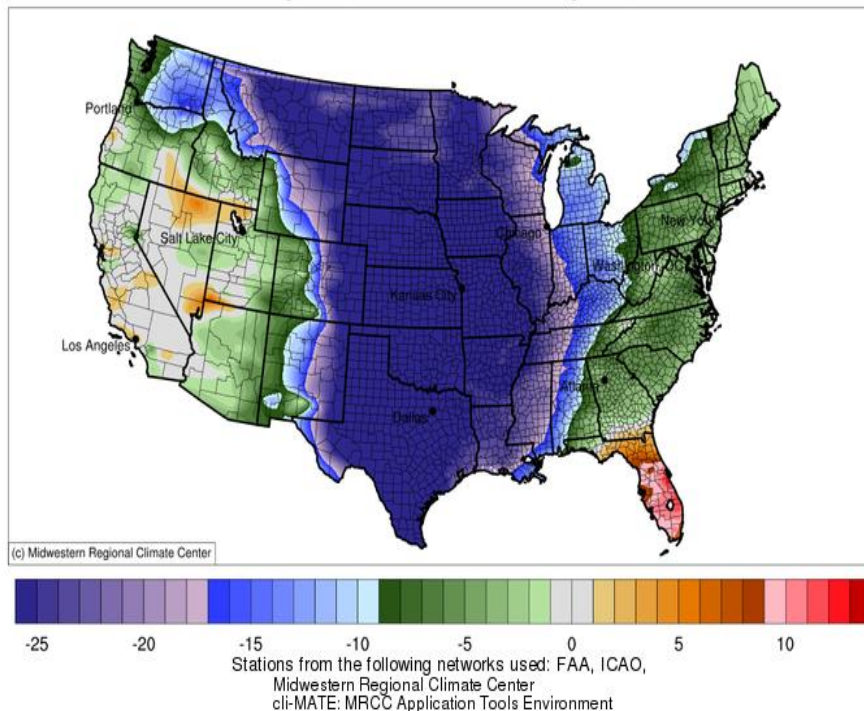
Average Temperature (°F): Departure from 1981-2010 Normals February 12, 2021 to February 18, 2021
