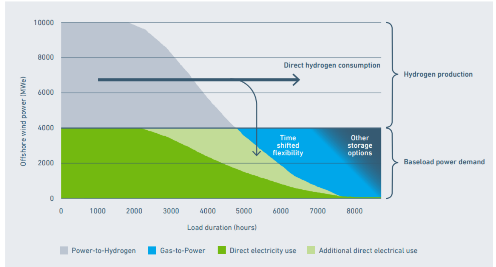
Figure 2b: Duration curve – grid-integrated scenario
