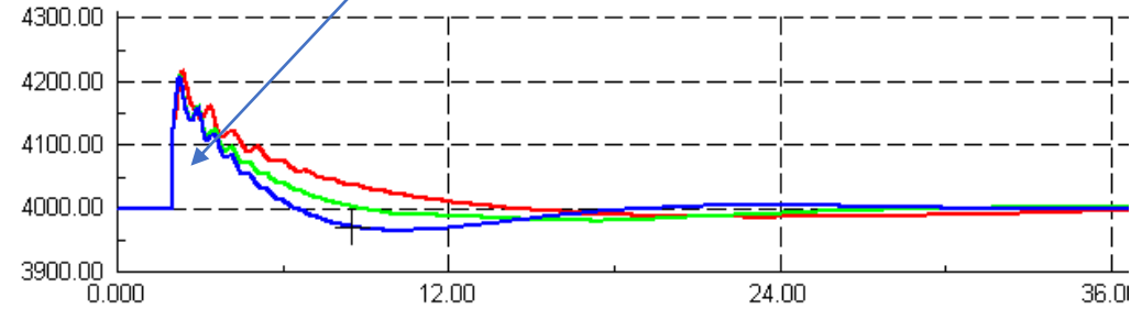
Active Power injection of Synchronous Plant during a fault/frequency fall
