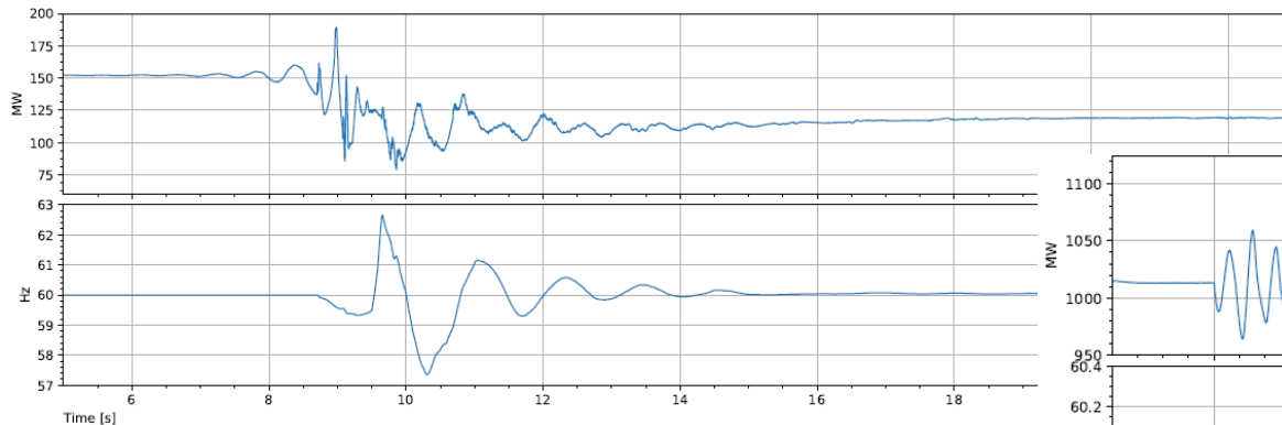
Maui GFL (instability followed by UFLS)
