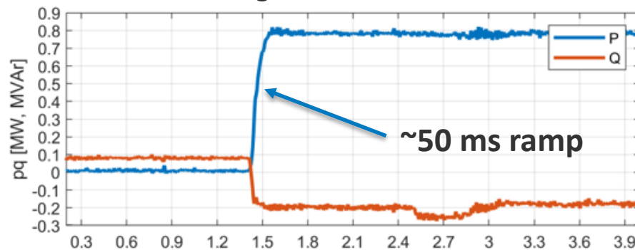
BESS Active and Reactive Power Response in Grid Forming Mode
