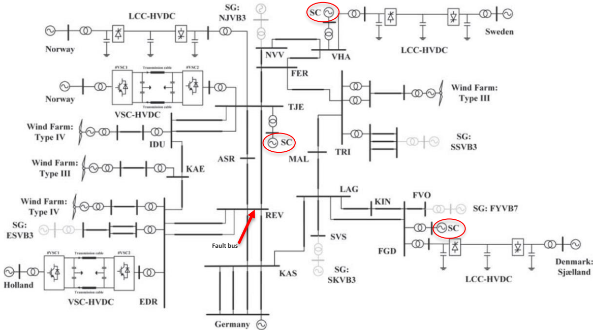
Simplified model of future Western Denmark power system (400 kV)
