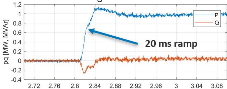
BESS Active and Reactive Power Response in Grid Following Mode
