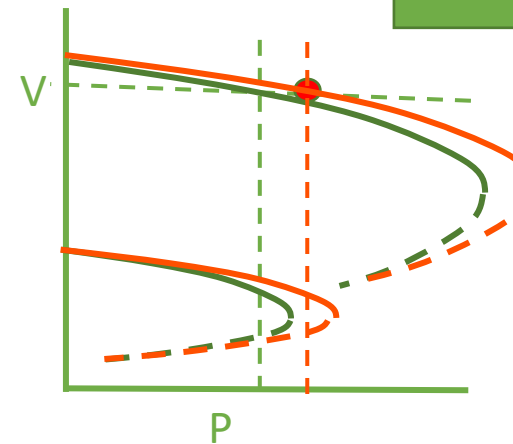
PV/Nose Curve
