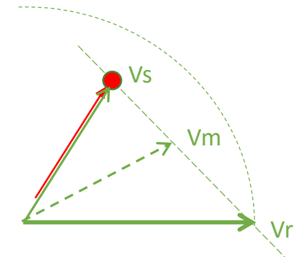
Phasor Diagram
