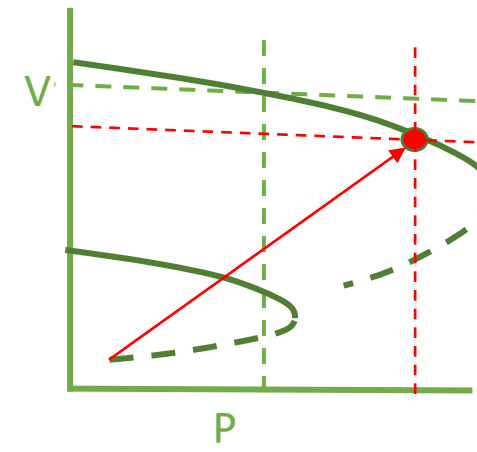
PV/Nose Curve
