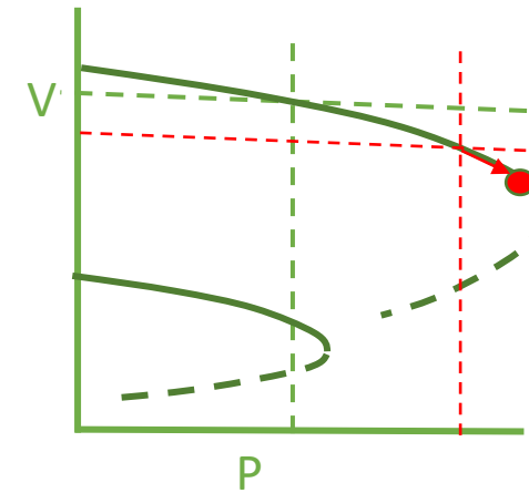
PV/Nose Curve
