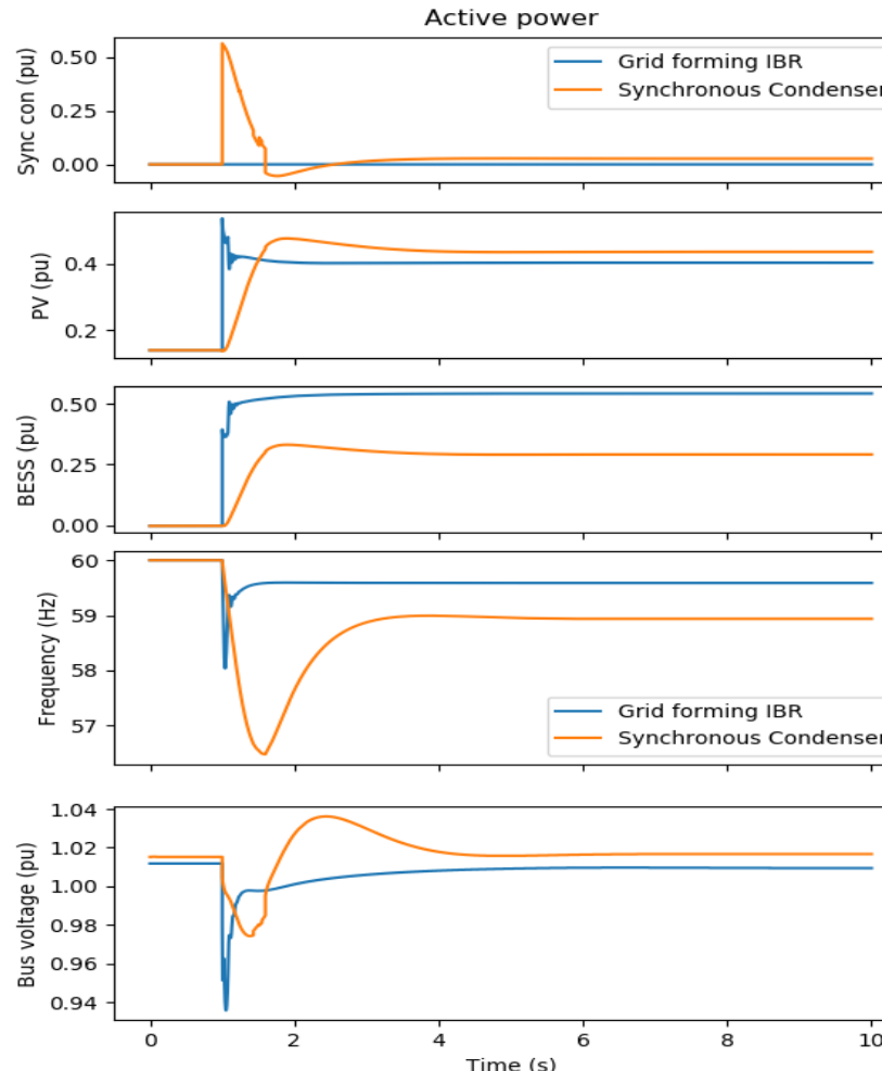
Extreme generation trip
