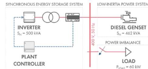
SMA Test System
