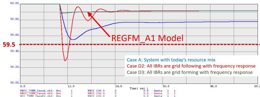
73% penetration of GFMs in the micro-WECC system
