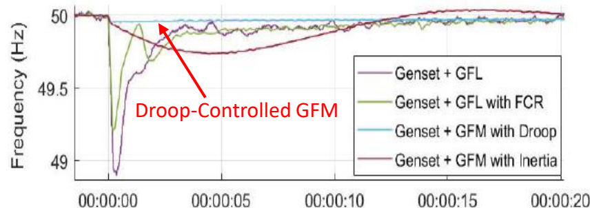
SMA Hardware Test Results [1]
