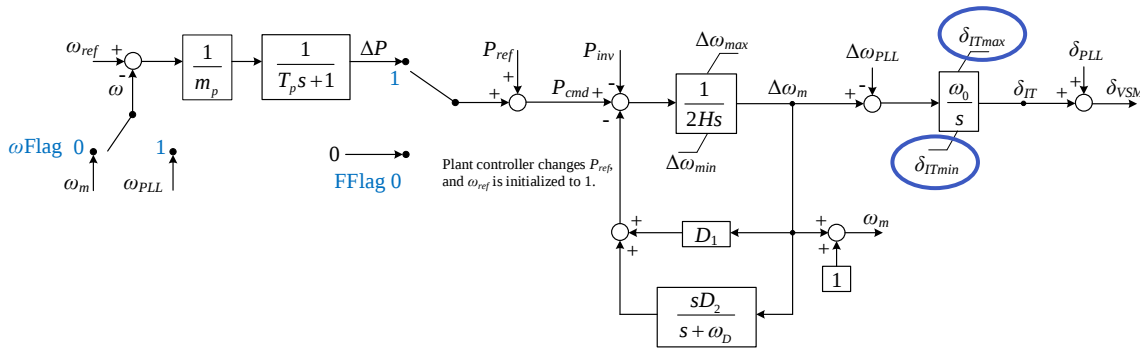
VSM/inertial control block
