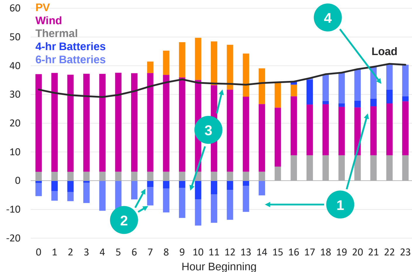
Illustrative high-renewables 24-hour dispatch GW of generation/load
