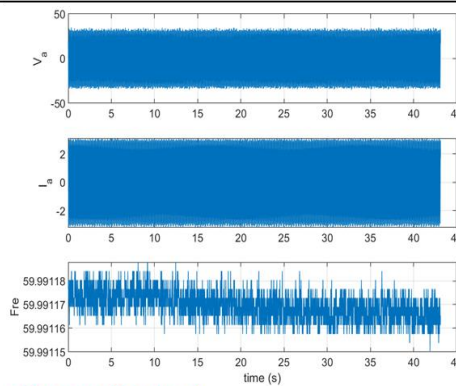
Frequency Generated from Droop Control
