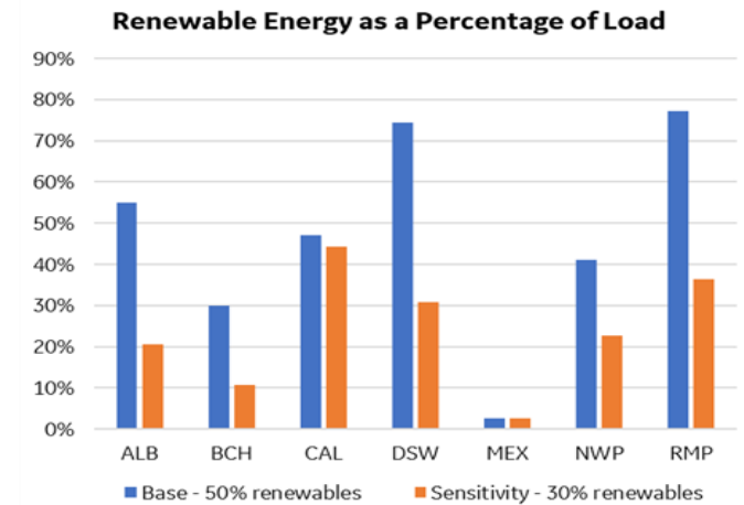
30% Renewable Penetration
