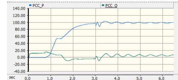
Example of “Small-Signal” Instability (P & Q)
