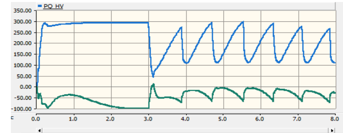
Example of “Large-Signal” Instability (P & Q)
