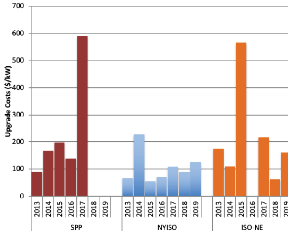
Figure 3: Trend in Generator Interconnection Network Upgrade Costs in SPP, NYISO, and ISO-NE ($/kW)
