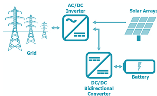
DC-Coupled Hybrid Plant
