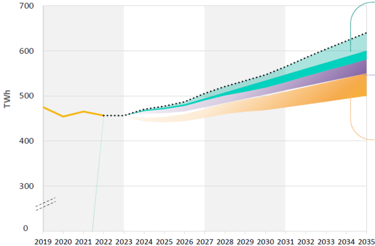
Evolution of electricity consumption in the different scenarios by 2035
