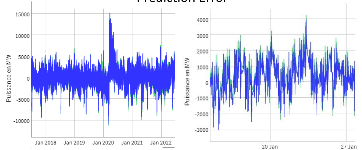
Prediction Error
