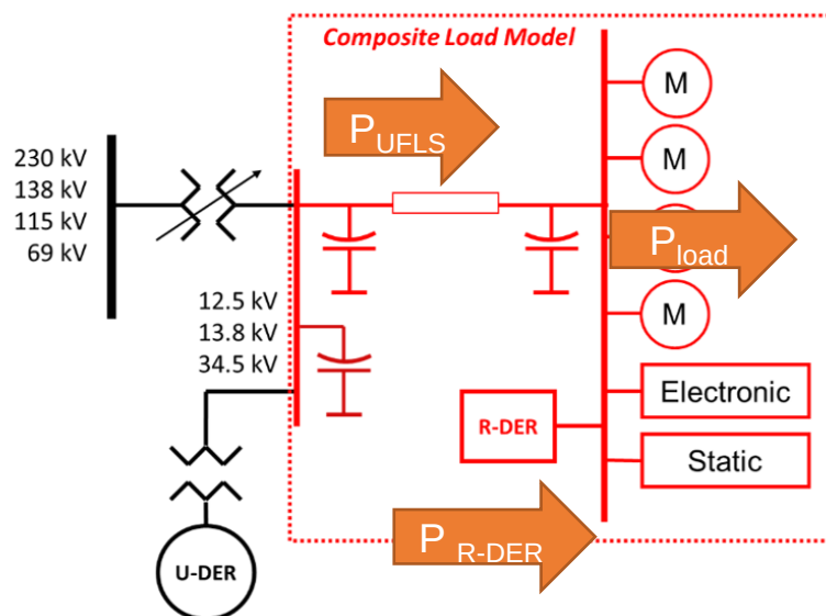
Figure 2.1: DER Modeling Framework
