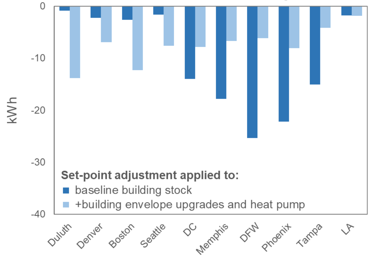
Reduction in Median Required Battery Size from Thermostat Set-Point Adjustments
