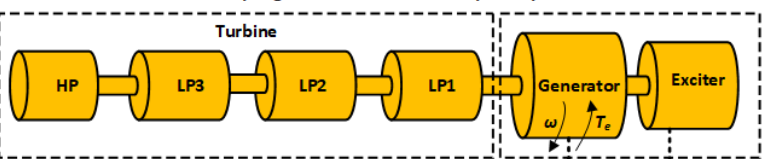
Spring mass model of thermal power plant
