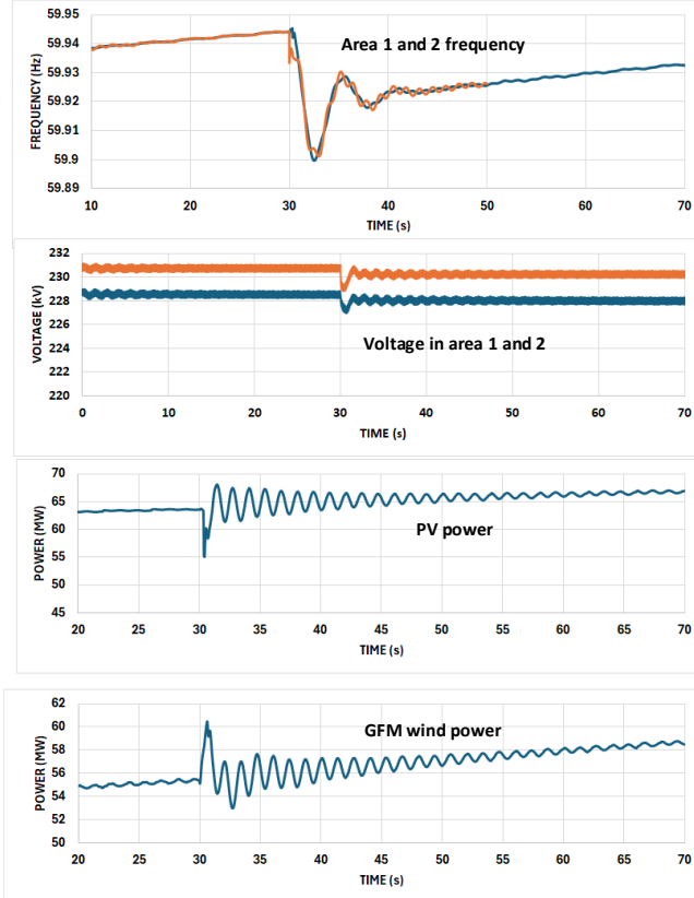
GFM wind and PV provide damping
