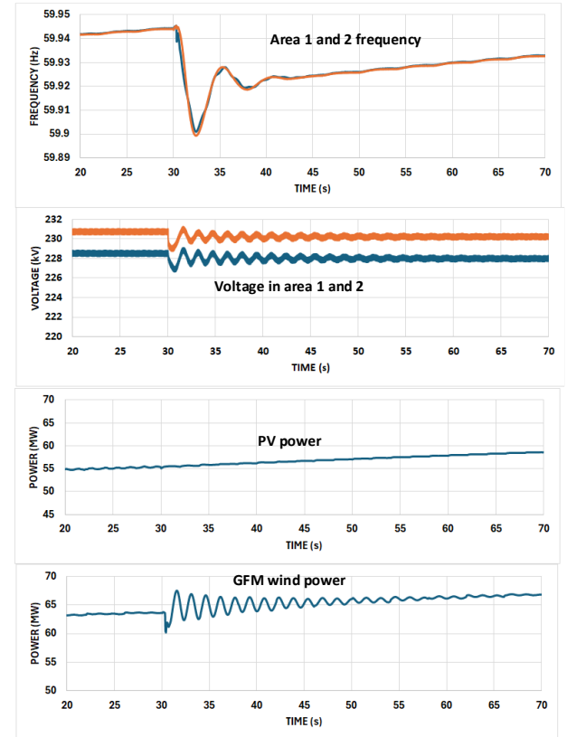
Only GFM provides damping
