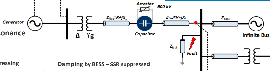
GFL BESS providing SSR damping control
