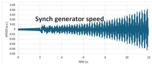
No damping by BESS – SSR progressing
