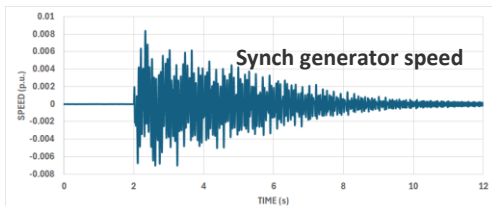
Damping by BESS – SSR suppressed
