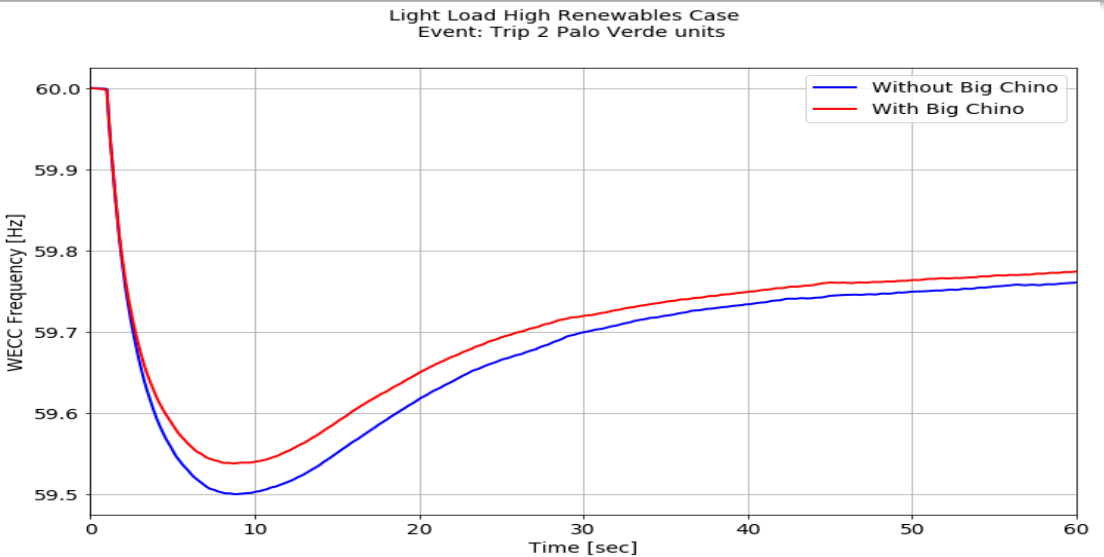
Frequency response margin and RoCoF without Big Chino
