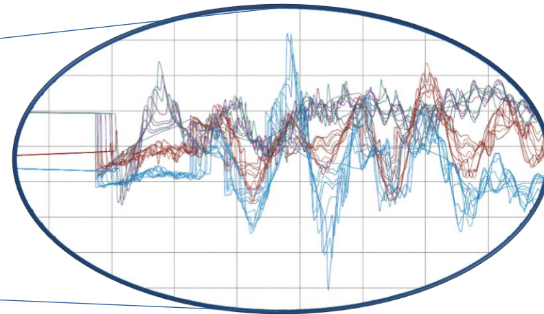
Capacitor breaker re-strike example
