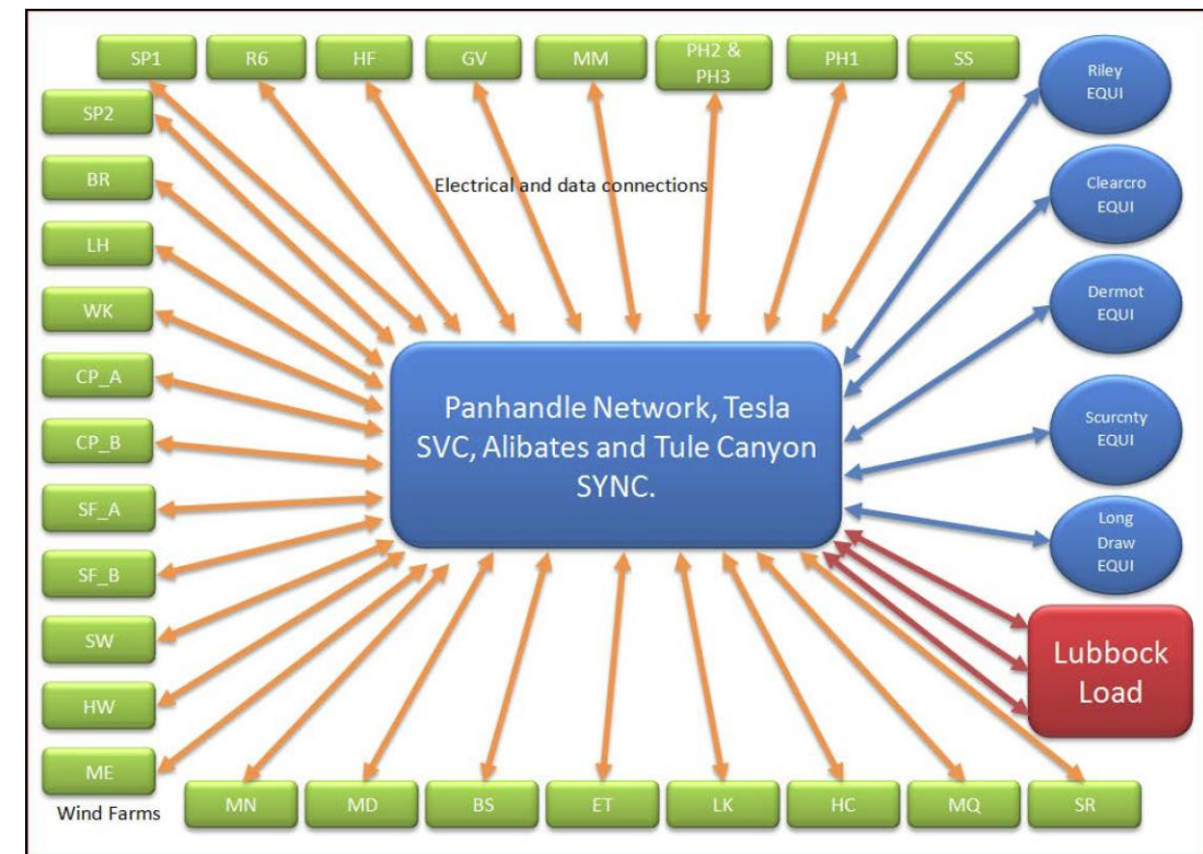
Parallel Simulation Example
