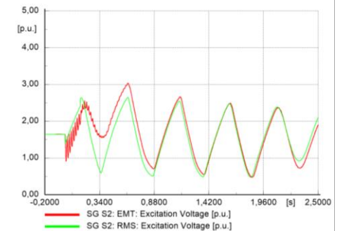
DigSILENT RMS-EMT Model Benchmarking
