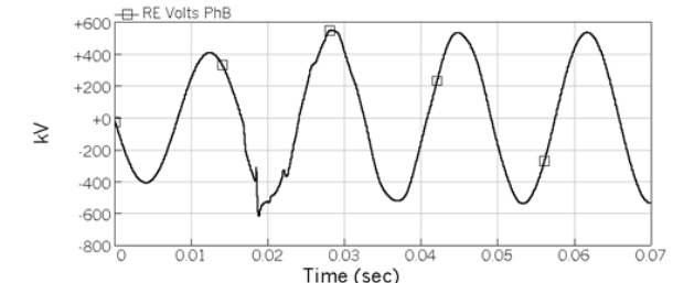
Frequency dependent (phase) model
