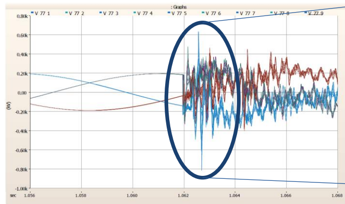
Capacitor breaker re-strike example
