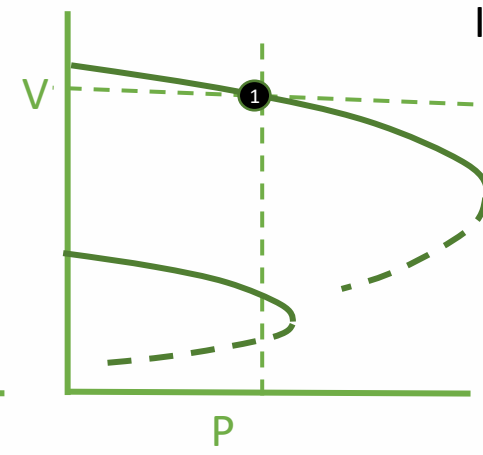
PV/Nose Curve
