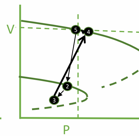
PV/Nose Curve
