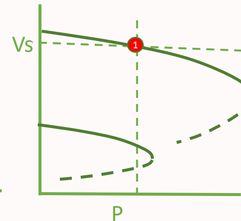
PV/Nose Curve
