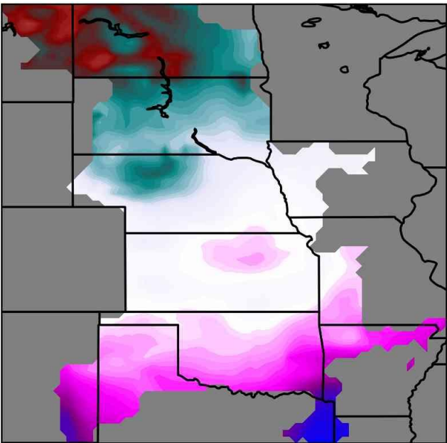
SPP ERA5 ANL 12z Wed Feb 19 25
