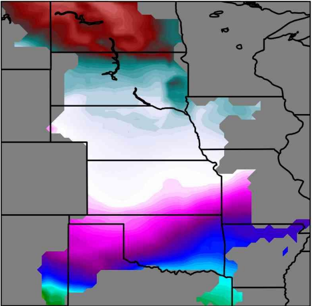
SPP ERA5 ANL 12z Tue Feb 18 25
