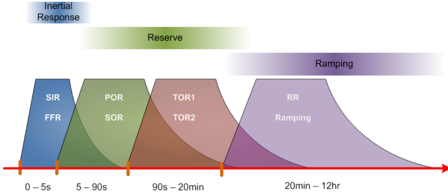
Figure 1: Frequency Control Services (Source: EirGrid)
