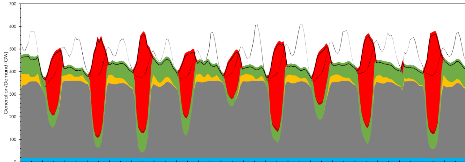
Example Summer Dispatch - 2050
