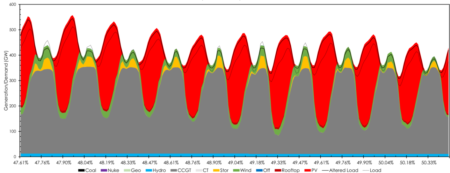
Example Summer Dispatch - 2050
