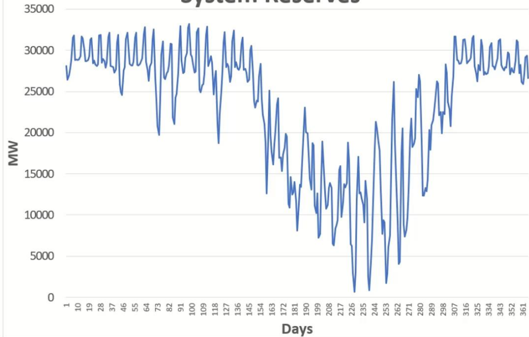
System Reserves
