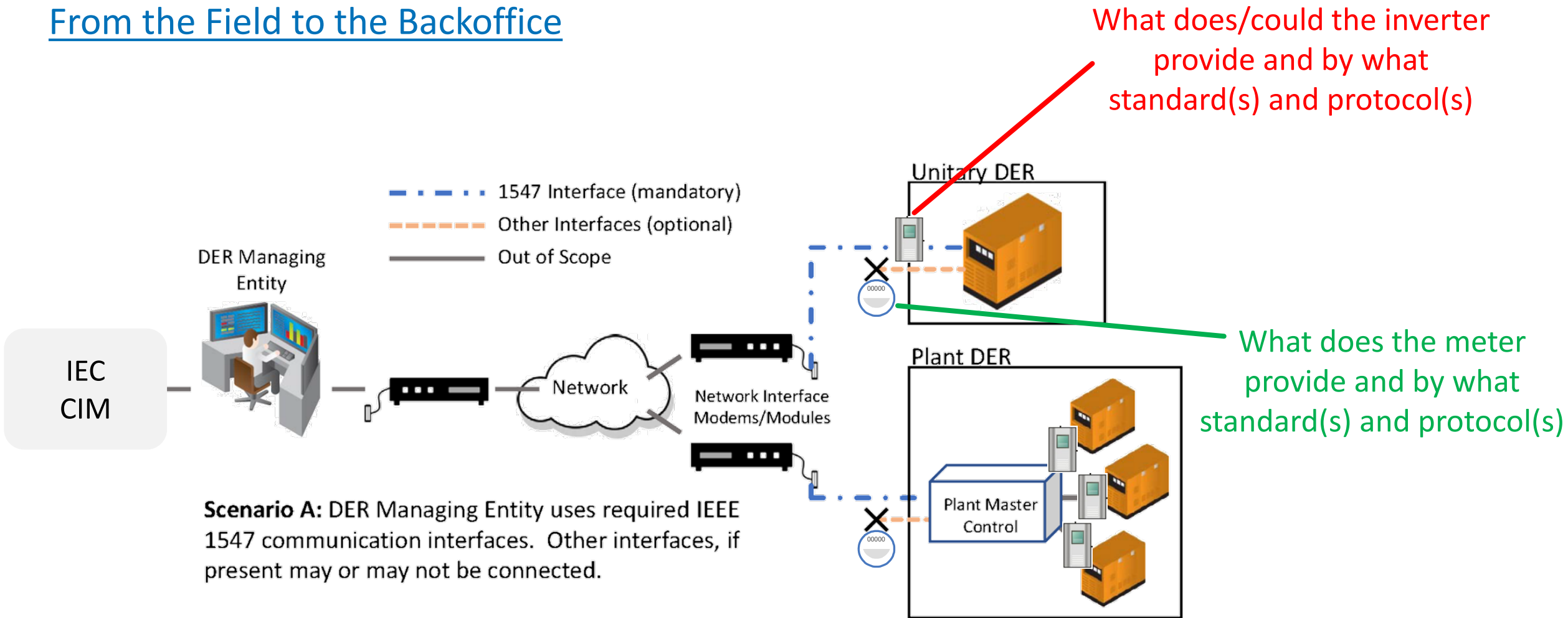
Figure D.1—DER using standardized local DER communication interface
