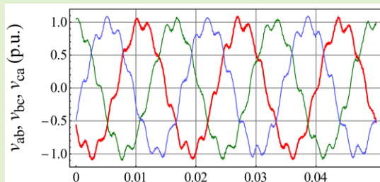
7-MVA grid simulator
