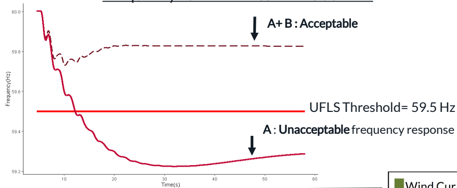
Frequency curve for loss of ~4500 MW
