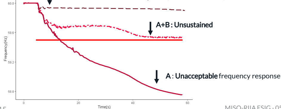
A+B + 6GW battery in EI (600 MW in MISO) : Sustained
