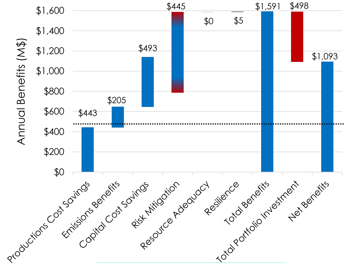
West Texas Export Option 2
