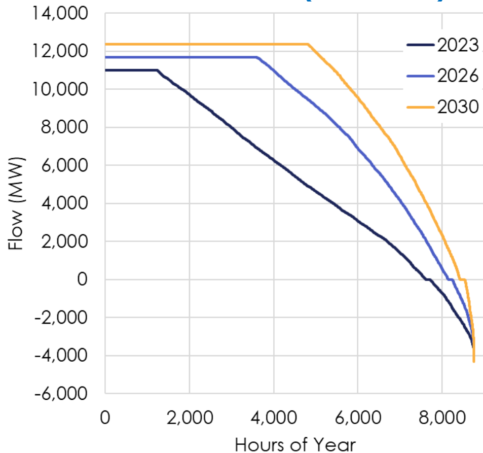
West Texas Export Interface Flow Duration Curve (Base Case)
