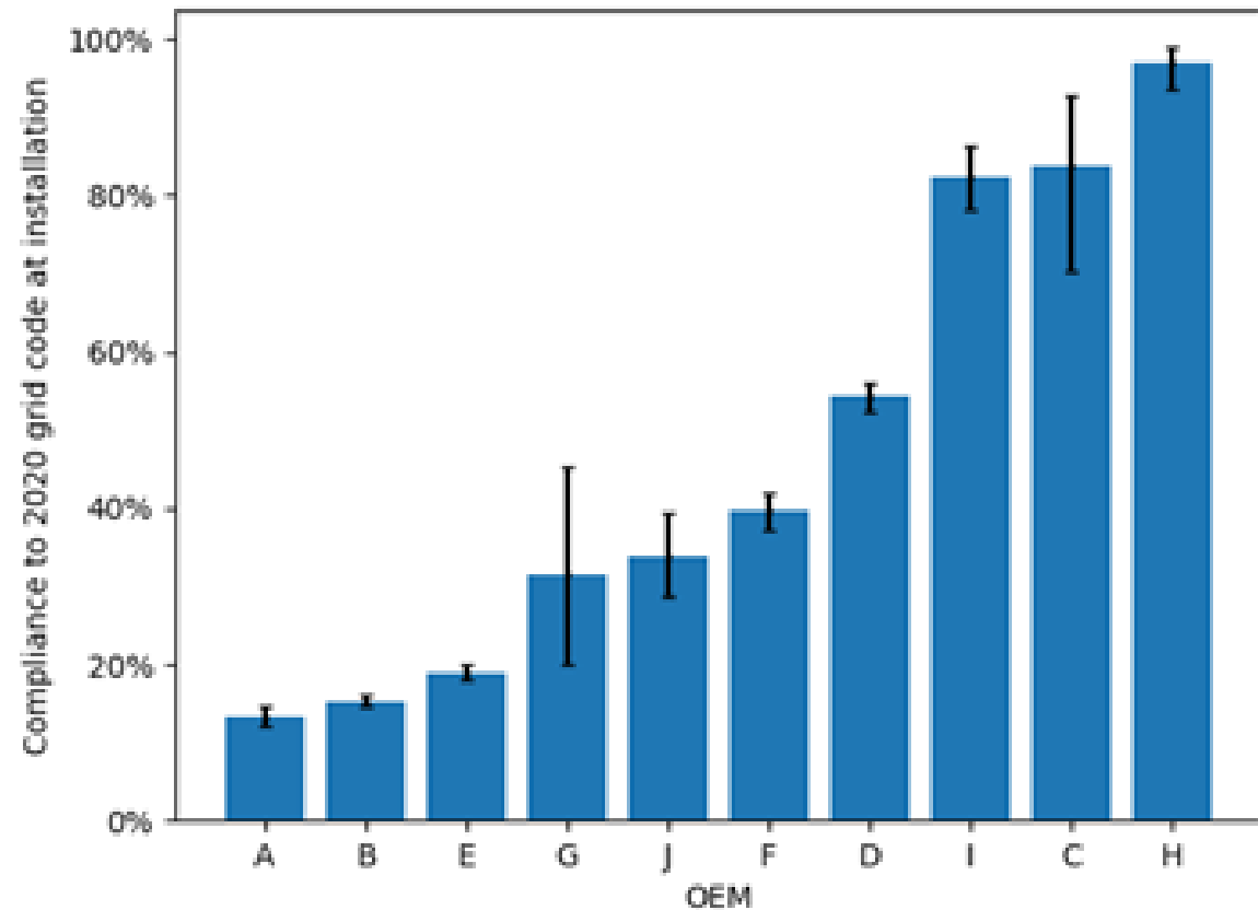
Compliance rates to 2020 standard (Q1 2022 installs in the NEM)
