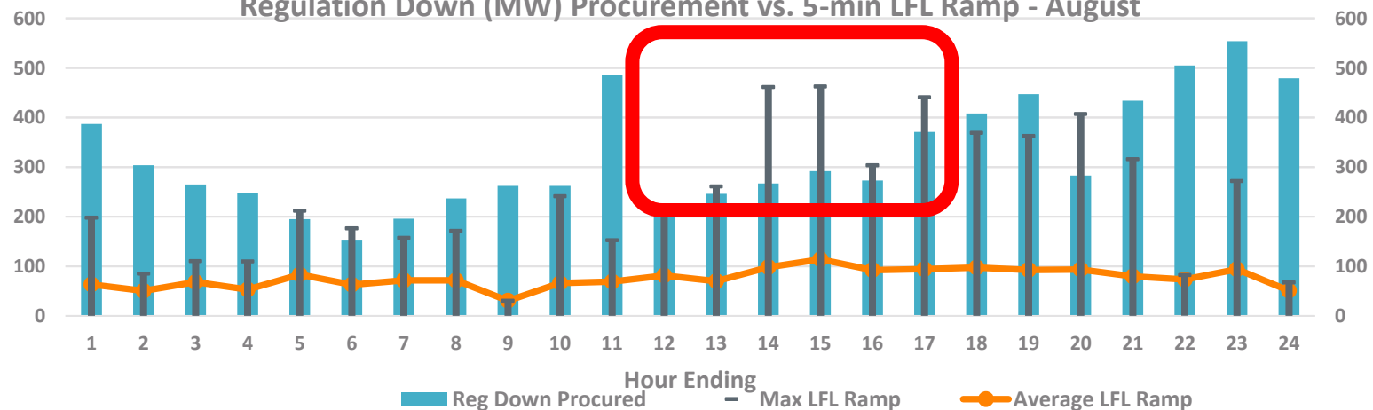
Regulation Down (MW) Procurement vs. 5-min LFL Ramp - August
