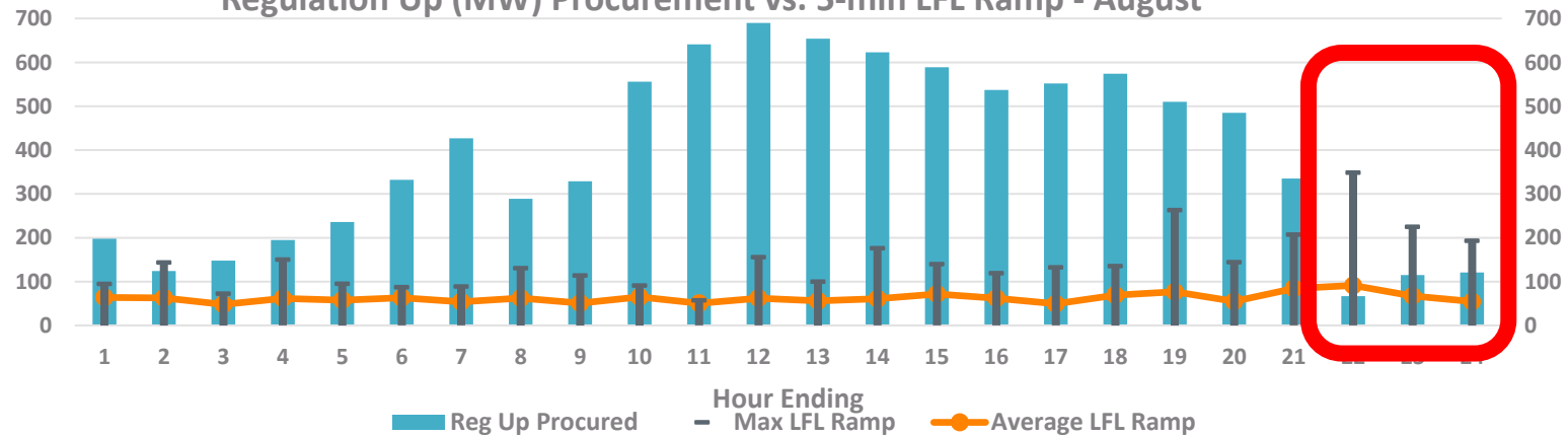
Regulation Up (MW) Procurement vs. 5-min LFL Ramp - August
