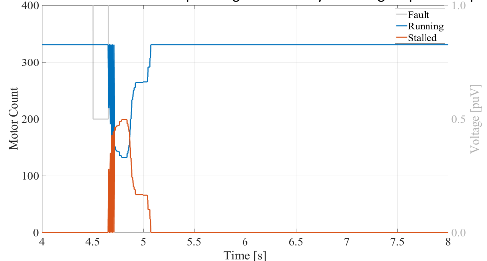
Residential Air Conditioner Operating States – 9-cycle voltage dip to 0.50 pu
