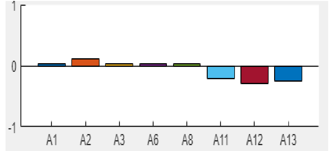
Impedance Participation Factor: Layer 2
