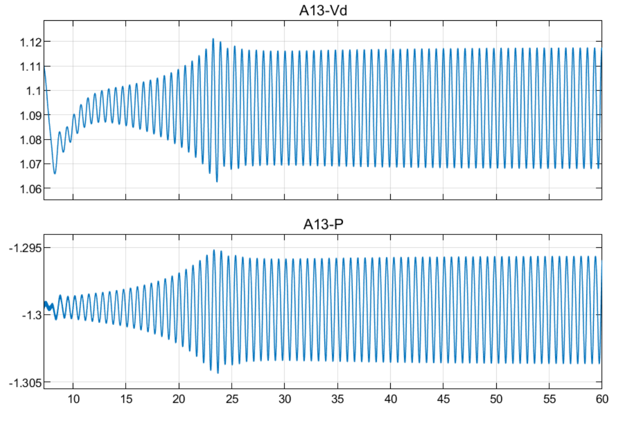
1.5 Hz free oscillation
