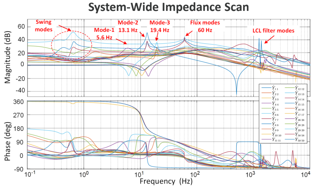
Identifying mode and impedance sensitivity from data
