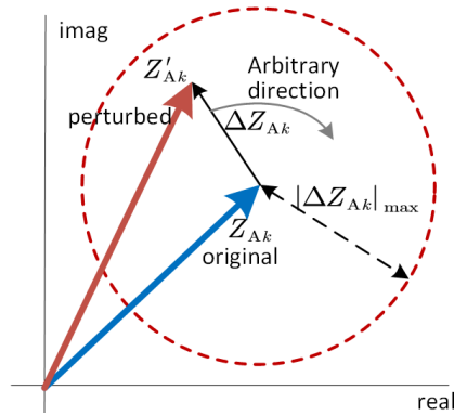
Impedance margin ( s=\lambda )
