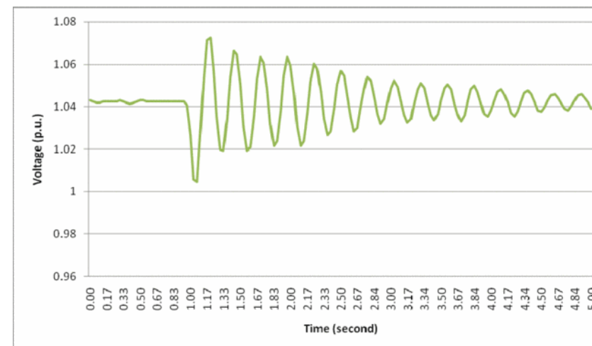
(a) Poorly-damped oscillation at low output
