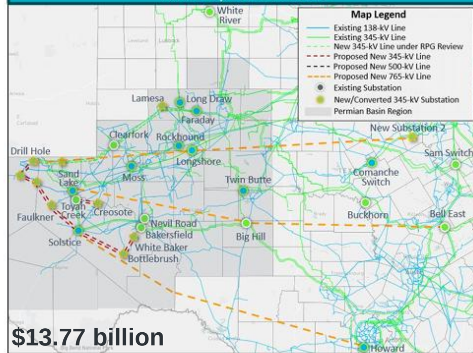
765-kV Import Paths in 2038
