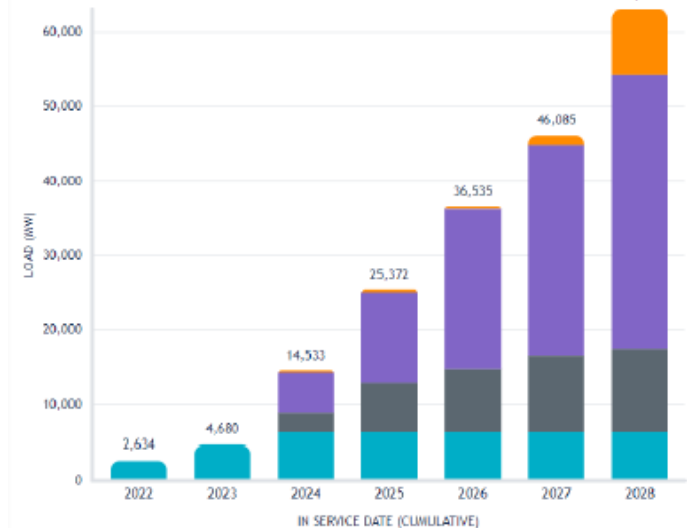
Actual and Projected Large Load Growth 2022-2028
