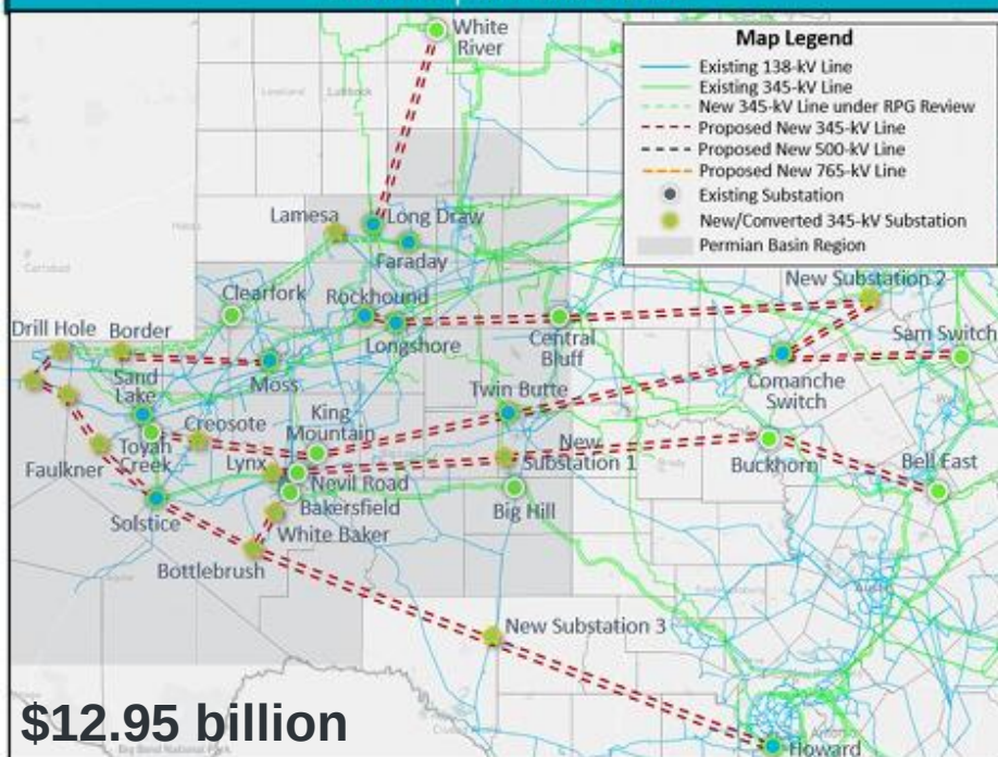
345-kV Import Paths in 2038
