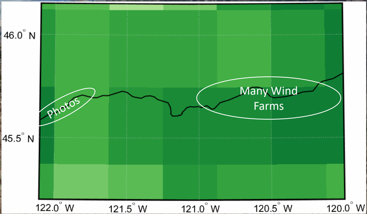
30 km Grid Spacing (~ERA5)
