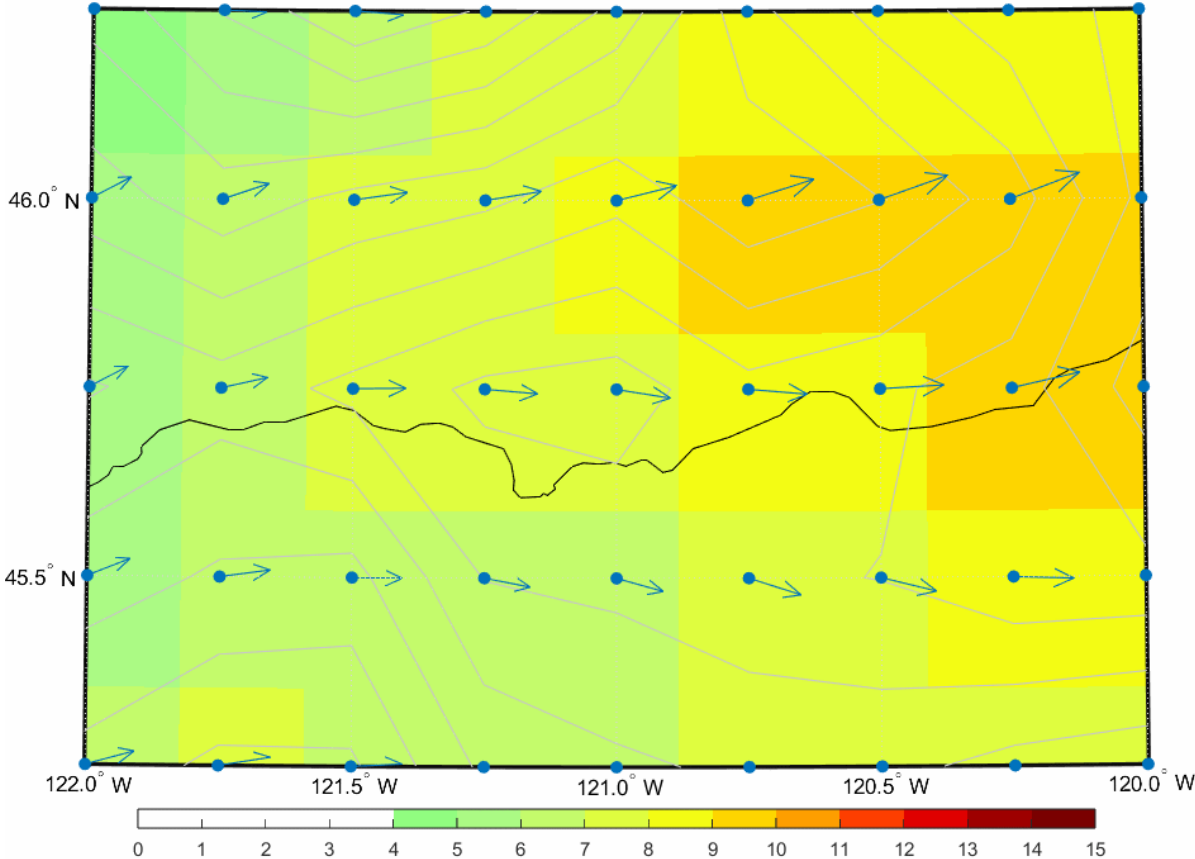
Windspeed and Vectors: 20100424:2100
