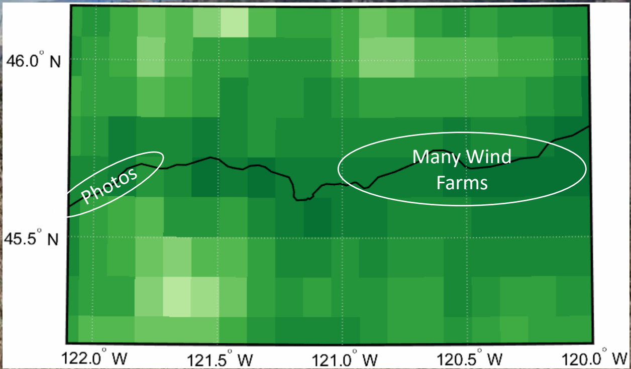
9 km Grid Spacing (~ECMWF)
