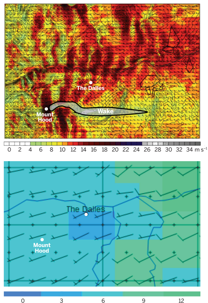
FIGURE 5 Wakes and Waves Observable in a 1 km, But Not 30 km, Simulation of the Columbia Gorge in the U.S. Pacific Northwest
