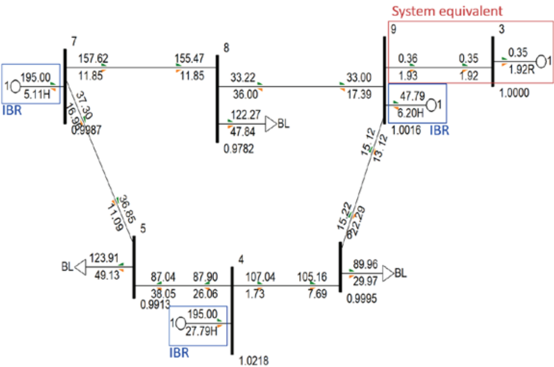
FIGURE A-1 A Test Network Used for Illustrating the Importance of Defining GFM Interconnection Requirements as Soon as Possible
