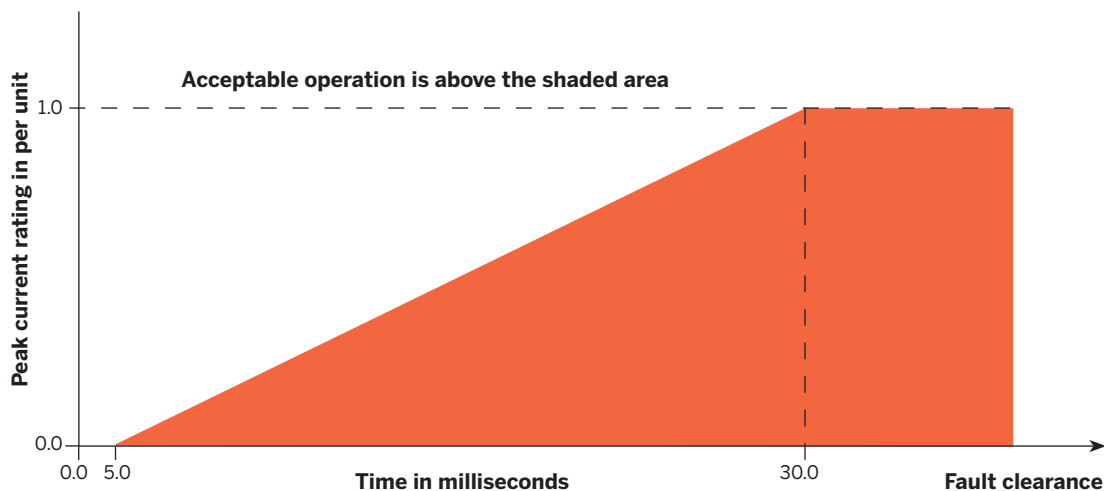
FIGURE 9 Injected Fault Current Rating Requirement for Grid-Forming Resources Under GC0137
