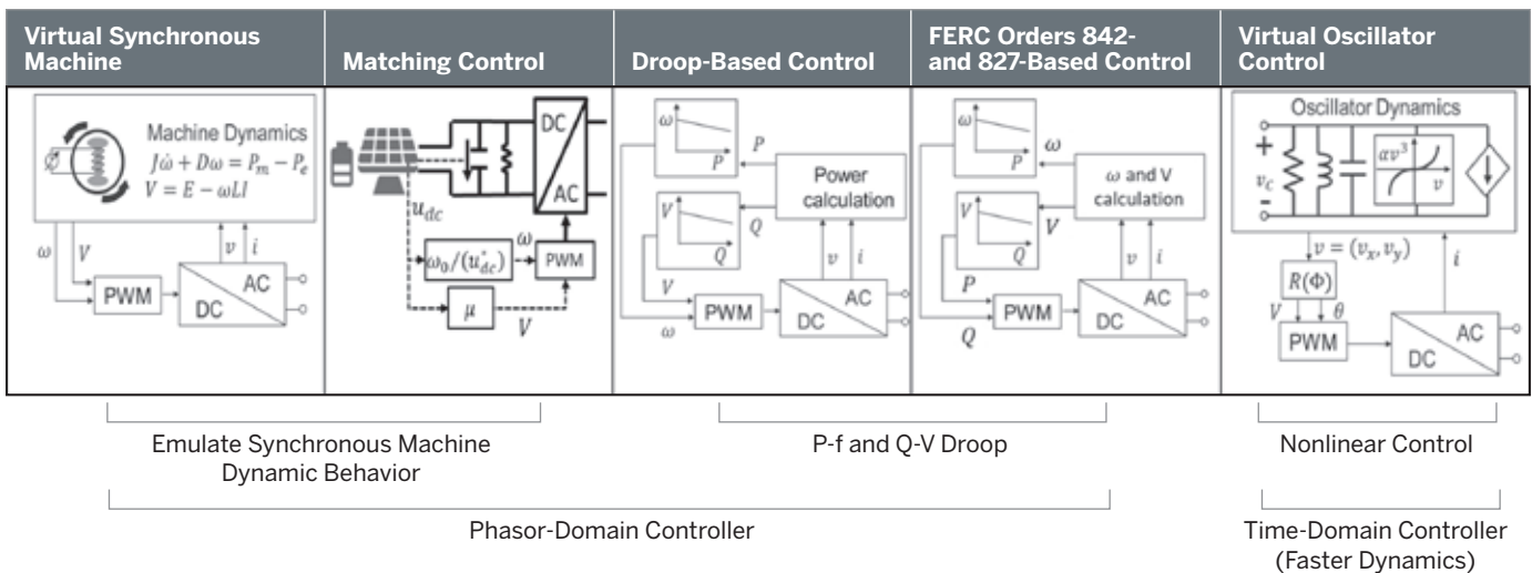
FIGURE 4 Proposed Control Concepts of Grid-Forming IBRs
