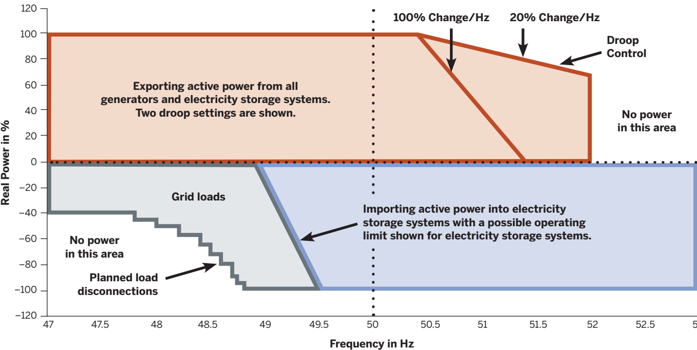
FIGURE 7 Power-Frequency Operating Characteristics of Grid-Forming Resources
